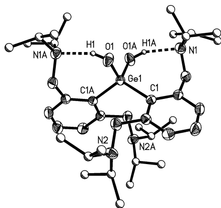
Figure 2. Structure of 6 (thermal ellipsoid level 50%); nonrelevant H atoms are omitted and i Pr groups are simplified for clarity. Selected bonds and angles: Ge1–O1 and Ge1–O1A 1.7522(11) Å, Ge1–C1 and Ge1–C1A 1.9668(16) Å, N1–O1 and N1A–O1A 2.737(3) Å, O1–Ge1–O1A 107.84(9)°, C1–Ge1–C1A 118.46(10)°.
