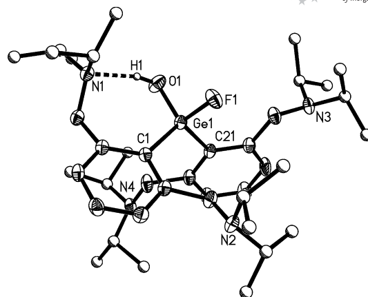
Figure 1. Structure of 2 (thermal ellipsoid level 50%); nonrelevant H atoms are omitted and i Pr groups are simplified for clarity. Selected bonds and angles: Ge1–O1 1.7363(12) \text{ \AA} , Ge1–F1 1.7543(10) \text{ \AA} , N1–O1 2.709(2) \text{ \AA} , O1–Ge1–F1 104.80(6)^\circ .
