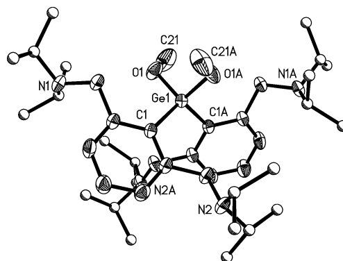
Figure 3. Structure of 1 (thermal ellipsoid level 50%); nonrelevant H atoms are omitted and i Pr groups are simplified for clarity. Selected bonds and angles: Ge1–O1 1.779(1) Å, Ge1–C1 1.965(2) Å, O1–Ge1–O1A 106.76(10)°, C1–Ge1–C1A 116.43(9)°.
